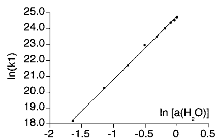
Figure 2. Linear fit of the logarithm of the proton ejection rate constant as a function of the logarithm of the water activity.
