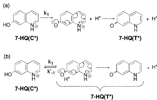
Figure 3. Scheme of the excited-state processes in 7-HQ(C*): (a) in [\text{HClO}_4] < 1 \text{ mol L}^{-1} solutions; (b) in [\text{HClO}_4] \geq 1 \text{ mol L}^{-1} solutions. k_1 is the proton ejection rate constant. k_{-1}' is the pseudo-first-order rate constant for proton recombination.
