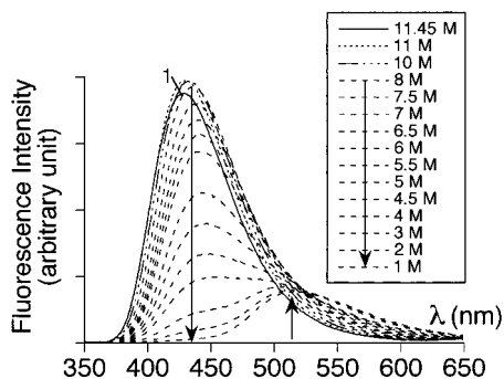
Figure 1. Corrected emission spectra of 7-HQ(C*) in aqueous perchloric solutions ( \lambda_{\text{exc}} = 340 nm). Spectrum 1 was recorded in 11.45 mol L -1 HClO 4 . The other spectra were recorded in progressively more diluted solutions.
